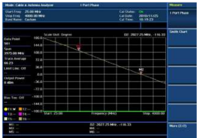
Cable and antenna test — 1-Port Phase
