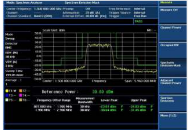
RF analysis — Spectrum Emission Mask
