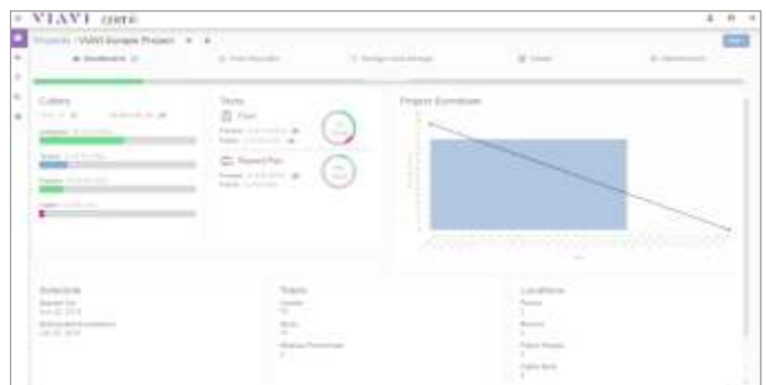
CERTiFi Dashboard
