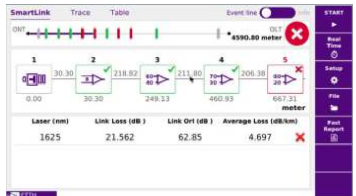
Unbalance/tap splitter network
