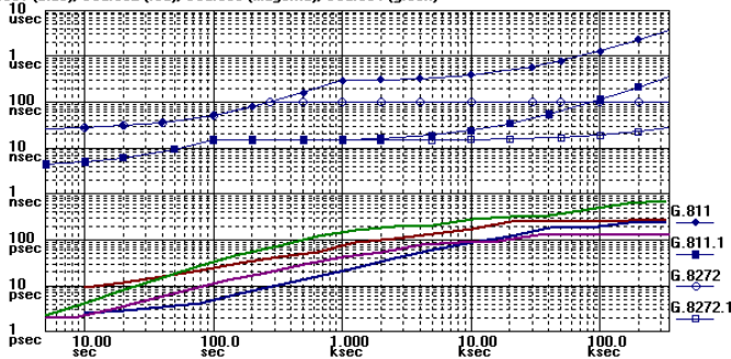
Four MTIE measurements compared to four telecom masks.
